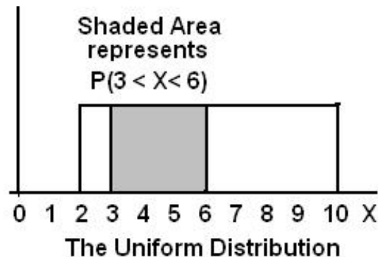
Figure 5.1: The graph shows a Uniform Distribution with the area between X=3 and X=6 shaded to represent the probability that the value of the random variable X is in the interval between 3 and 6.
